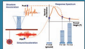
Spectral Acceleration: Buildings of different heights respond differently to the same ground motion because they have different vibrational periods
